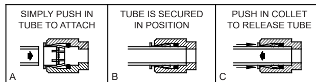
Figure 20 – Quick Connect Fittings
