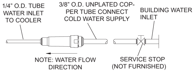
Figure 4 – Water Supply Connections
