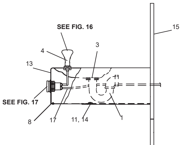
Figure 18 – Fountain Assembly - Side View
