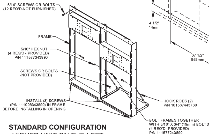
Figure 6 – Rough-In Assembly Dual-Station Mounting Frames
