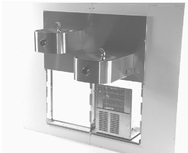
Figure 13 – HRFSER Fountain Installation
