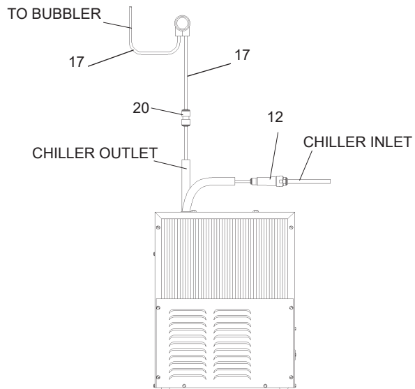
Figure 19 – HRFER/HRFSR Tube Routing
