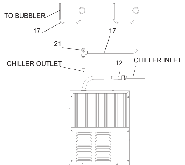
Figure 15 – HRFSER/HRFESR Tube Routing
