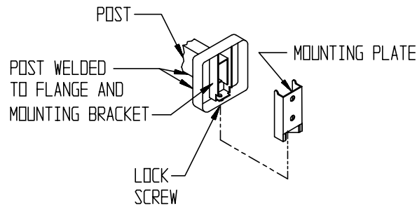
CONCEALED MOUNTING DETAIL
