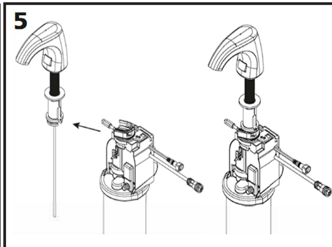
5 Slide Pump Assembly onto pump extender.
