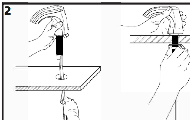
2 Insert Spout into counter hole. Align the Spout in the desired position. From the underside of the counter, assemble the Washer, then the nut onto the Stem and tighten. For proper installation, counter thickness cannot exceed 2-5/8".
