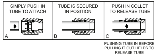
Fig 6: Poly Tube Quick Connect Fitting
