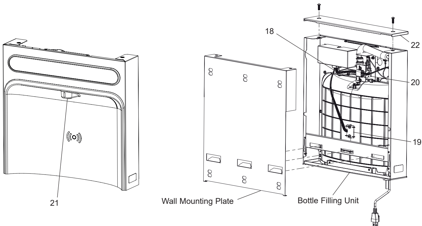
Fig 5: Front View with Aerator
