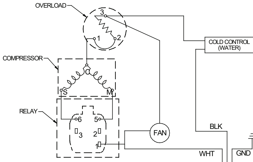
Fig 8: 115V Wiring Diagram
