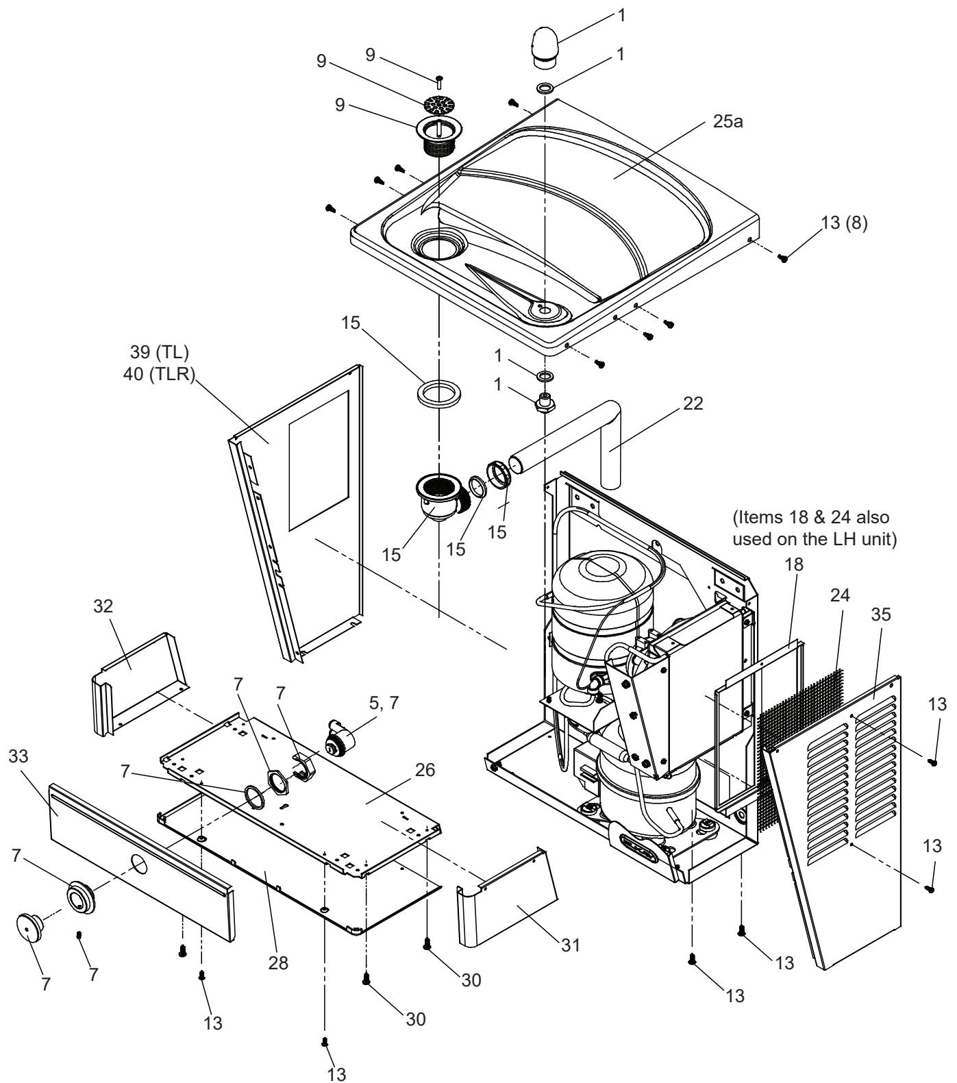
FIG. 8 (Refrigerated side shown)
