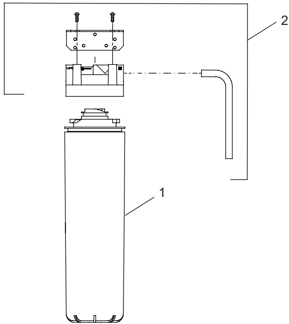
WATER FILTER EXPLODED VIEW
