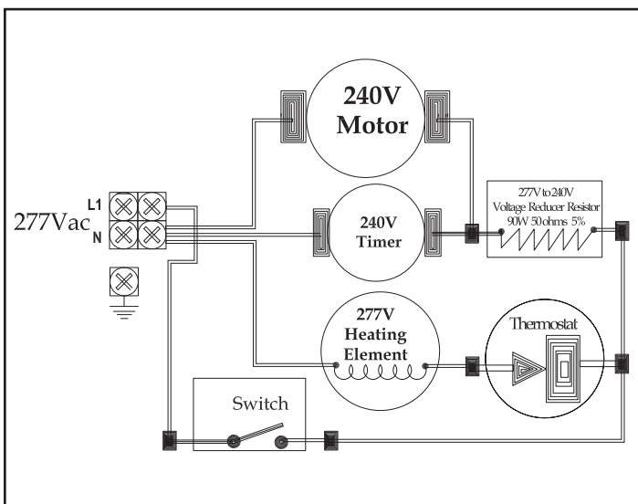
Wiring Diagram - Model RA57
