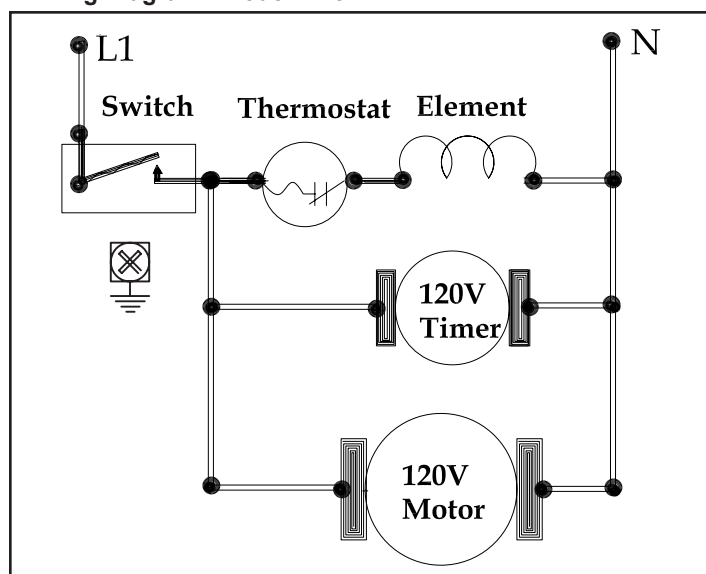
Wiring Diagram - Model RA5
