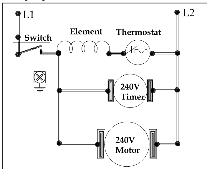
Wiring Diagram - Model RA54/RA548
