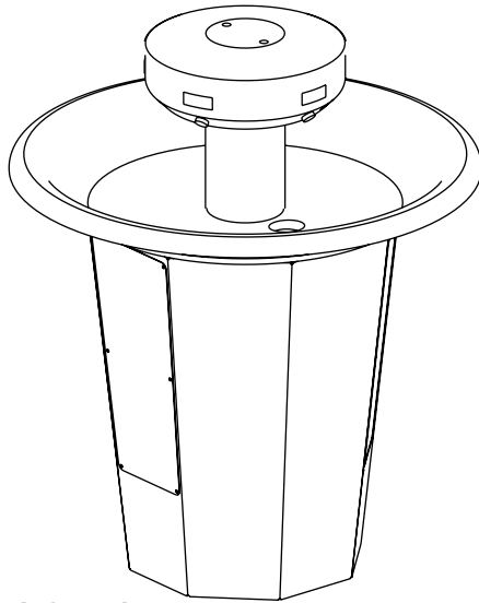
SN2005 - Infrared
