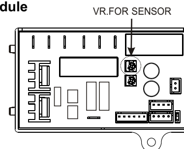
VR.FOR SENSOR
